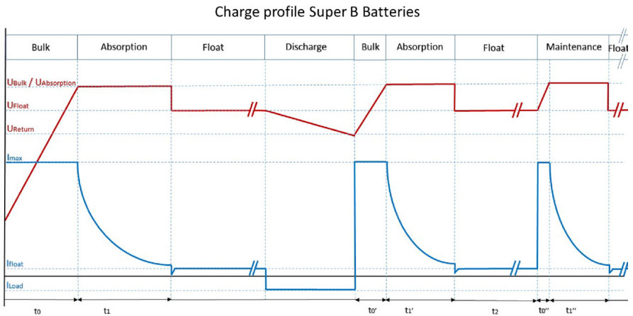
Figure 1. Charge profile Super B Batteries
